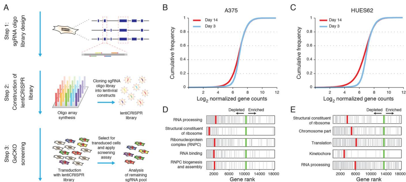
Fig. 2. GeCKO library design and application for genome-scale negative selection screening. (A) Design of sgRNA library for genome-scale knockout of coding sequences in human cells (supplementary discussion). (B and C) Cumulative frequency of sgRNAs 3 and 14 days post transduction in A375 and hES cells respectively. Shift in the 14 day curve represents the depletion in a subset of sgRNAs. (D and E) Five most significantly depleted gene sets in A375 cells (nominal P < 10^{-5} , FDR-corrected q < 10^{-5} ) and HUES62 cells (nominal P < 10^{-5} , FDR-corrected q < 10^{-3} ) identified by Gene Set Enrichment Analysis (GSEA) (15).
