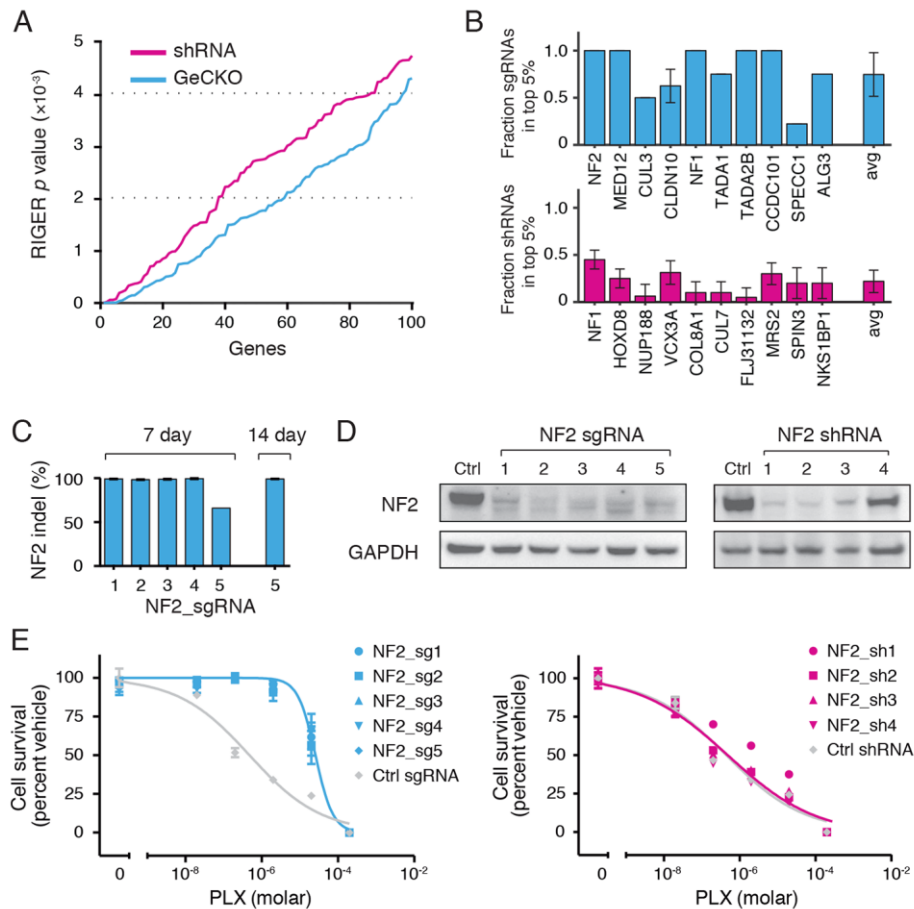
Fig. 4. Comparison of GeCKO and shRNA screens and validation of neurofibromin 2 ( NF2 ). (A) RIGER P values for the top 100 hits from GeCKO and shRNA (19) screens for genes whose loss results in PLX resistance. Analysis using the Redundant siRNA Activity (RSA) algorithm shows a similar trend (fig. S9). (B) For the top 10 RIGER hits, the percent of unique sgRNAs (top) or shRNAs (bottom) targeting each gene that are in top 5% of all enriched sgRNAs or shRNAs. (C) Deep sequencing analysis of lentiCRISPR-mediated indel at the NF2 locus. (D) A375 cells transduced with NF2 -targeting lentiCRISPR and shRNA vectors both show a decrease in NF2 protein levels. (E) Dose response curves for A375 cells transduced with individual NF2 -targeting lentiCRISPR or shRNA vectors. Controls were EGFP-targeting lentiCRISPR or null hairpin shRNA vectors. Cells transduced with NF2 -targeting lentiCRISPRs show a significant increase ( F_{1,8} = 30.3 , P < 0.001 , n = 4 replicates) in the half maximal effective concentration ( EC_{50} ) whereas cells transduced with NF2 -targeting shRNA vectors do not ( F_{1,8} = 0.47 , P = 0.51 , n = 4 replicates).
