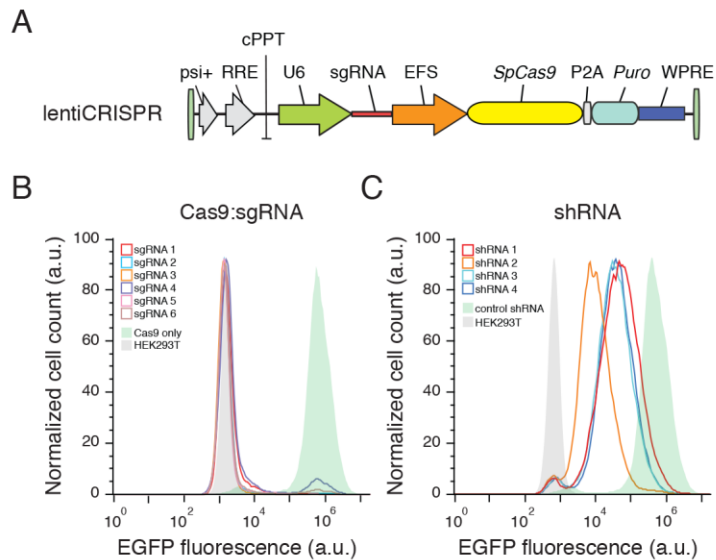
Fig. 1. Lentiviral delivery of Cas9 and sgRNA provides efficient depletion of target genes. (A) Lentiviral expression vector for Cas9 and sgRNA (lentiCRISPR). Puromycin selection marker (puro), psi packaging signal (psi+), rev response element (RRE), central polypurine tract (cPPT), elongation factor-1 \alpha short promoter (EFS), 2A self-cleaving peptide (P2A), and posttranscriptional regulatory element (WPRE). (B) Distribution of fluorescence from 293T-EGFP cells transduced by EGFP-targeting lentiCRISPR (sgRNAs 1-6, outlined peaks) and Cas9-only (green-shaded peak) vectors, and non-fluorescent 293T cells (gray shaded peak). (C) Distribution of fluorescence from 293T-EGFP cells transduced by EGFP-targeting shRNA (shRNAs 1-4, outlined peaks) and control shRNA (green-shaded peak) vectors, and non-fluorescent 293T cells (gray shaded peak).
